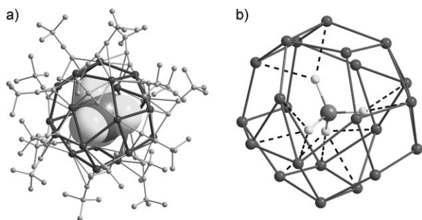
Figure 2. a) Structure of the cationic part of [\text{Ag}_{22}(\text{C}\equiv\text{tBu})_{18}(\text{CrO}_4)](\text{BF}_4)_2 1 . The templating chromate ion is shown in space-filling mode. Hydrogen atoms and Ag–O bonds are omitted for clarity. b) Ball-shaped core structure in 1 .
